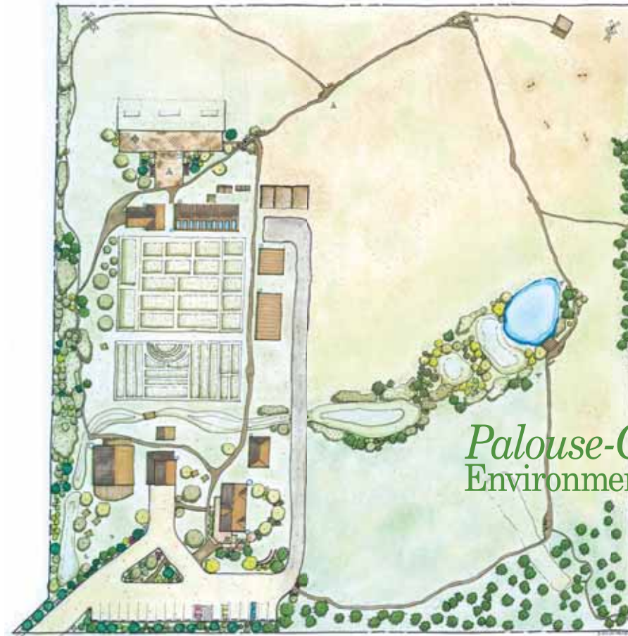
1"=20' PCEI RODEO DRIVE MASTERPLAN
